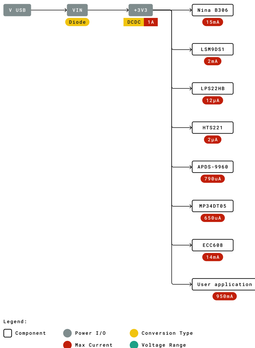
Power tree
